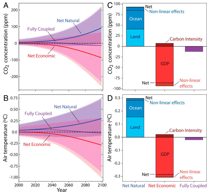
Fig. 2. Net effects of including only natural, only economic, or both sets of feedbacks in our model compared with the baseline (no feedbacks) scenario. All values shown are given as the difference between the baseline and that scenario. (A and B) Air temperature and atmospheric CO 2 over the 21st century with uncertainty bounds on the fully coupled and net economic scenarios. Natural carbon–climate feedbacks (net natural) increased atmospheric CO 2 and temperature, whereas economic feedback processes (net economic) decreased them. The net economic effect more than offset the net natural, so the fully coupled scenario showed an overall negative effect on temperature and atmospheric CO 2 . (C and D) The change in temperature and atmospheric CO 2 from 1800 to 2100 for these scenarios along with decompositions of the contributions to each net effect. For the natural carbon cycle, effects from the land and ocean in our model were similar in magnitude. Temperature effects on GDP drove the net economic effect strongly down, and although the carbon intensity of energy (carbon intensity) response caused a slight increase, the overall effect was dominated by GDP. Both net natural and net economic simulations also had some nonlinear interaction effects that were not captured by our decoupled scenarios.
